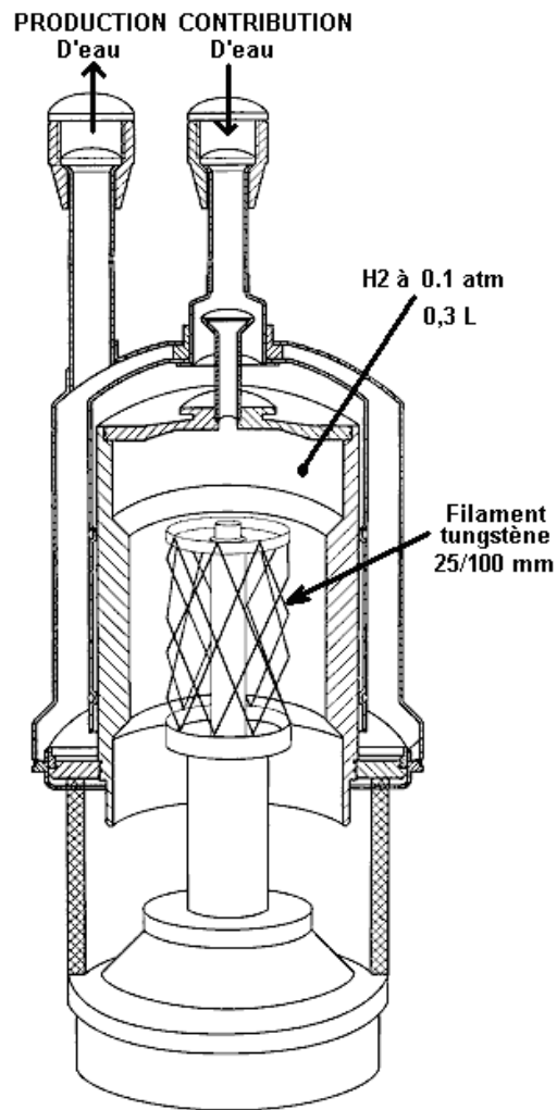
Le MAHG (Moller Atomic Hydrogen Generator)
