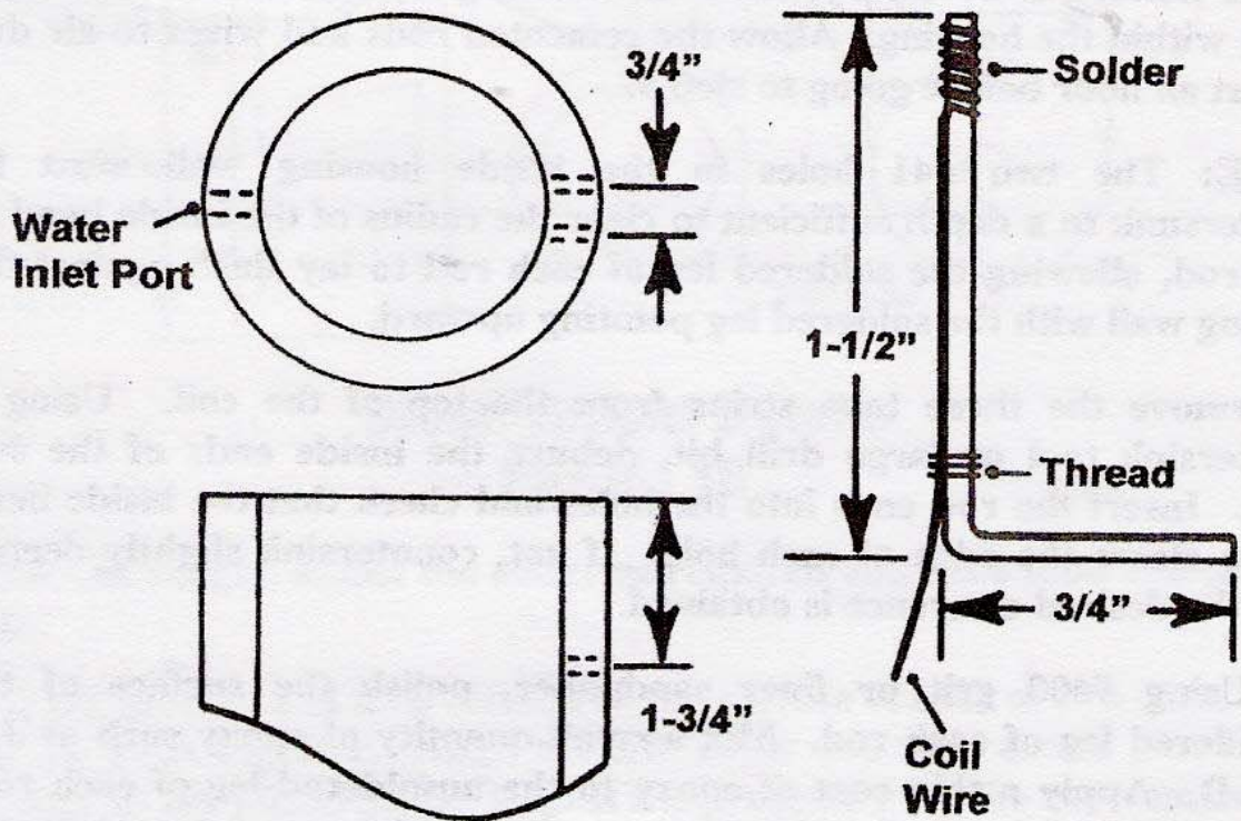
Toroid Coil Installation Figure 20
