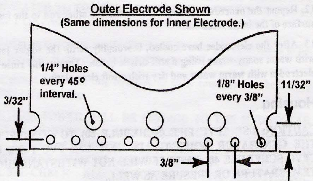
Electrode Details Figure 8
