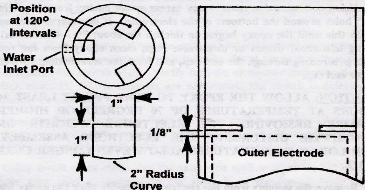
Coil Mounting Brackets Figure 12
