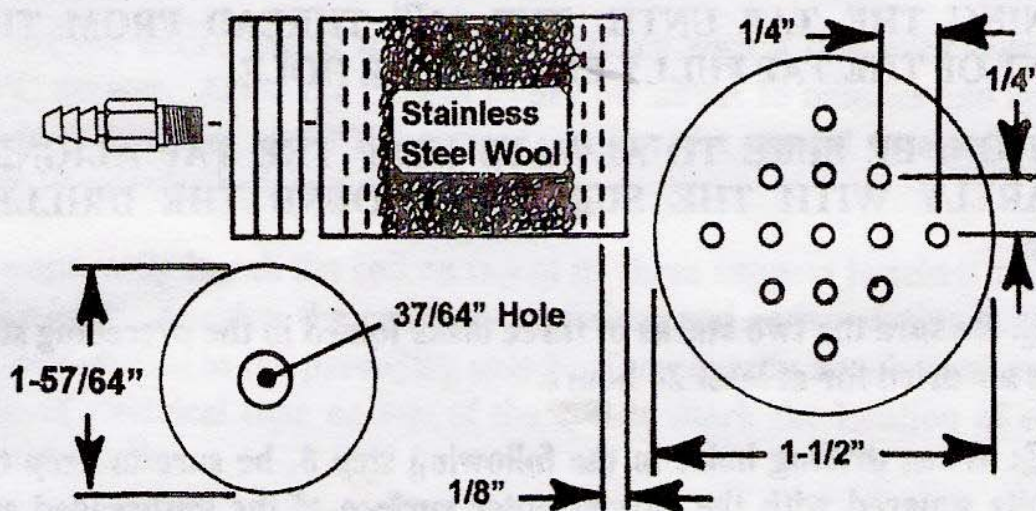
Flame Arrestor Details Figure 17
