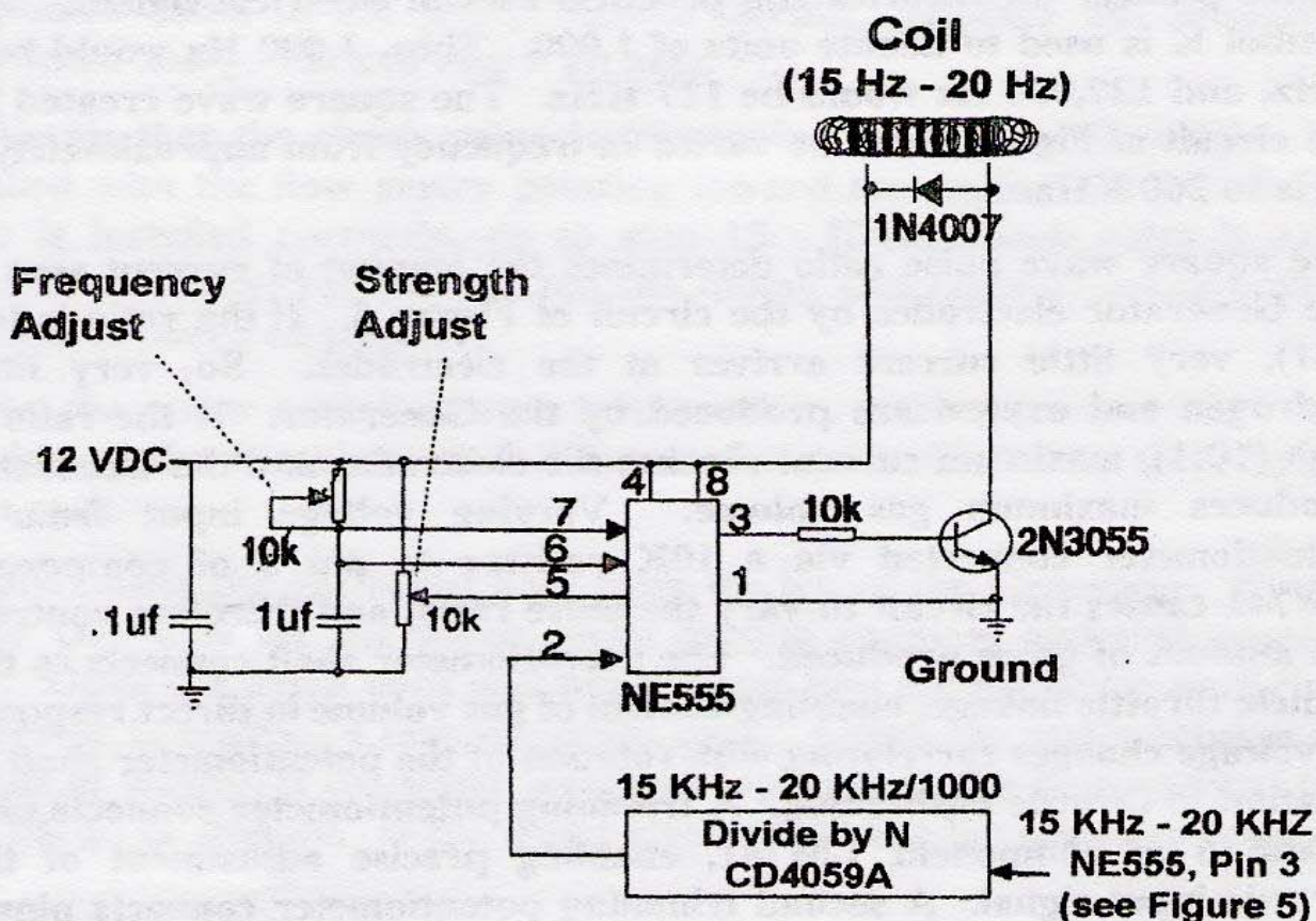
Generator Coil Circuit Schematic Figure 6
