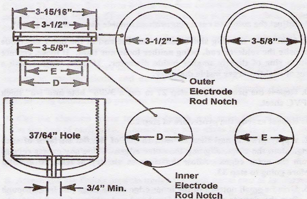
Threaded End Cap Details Figure 11
