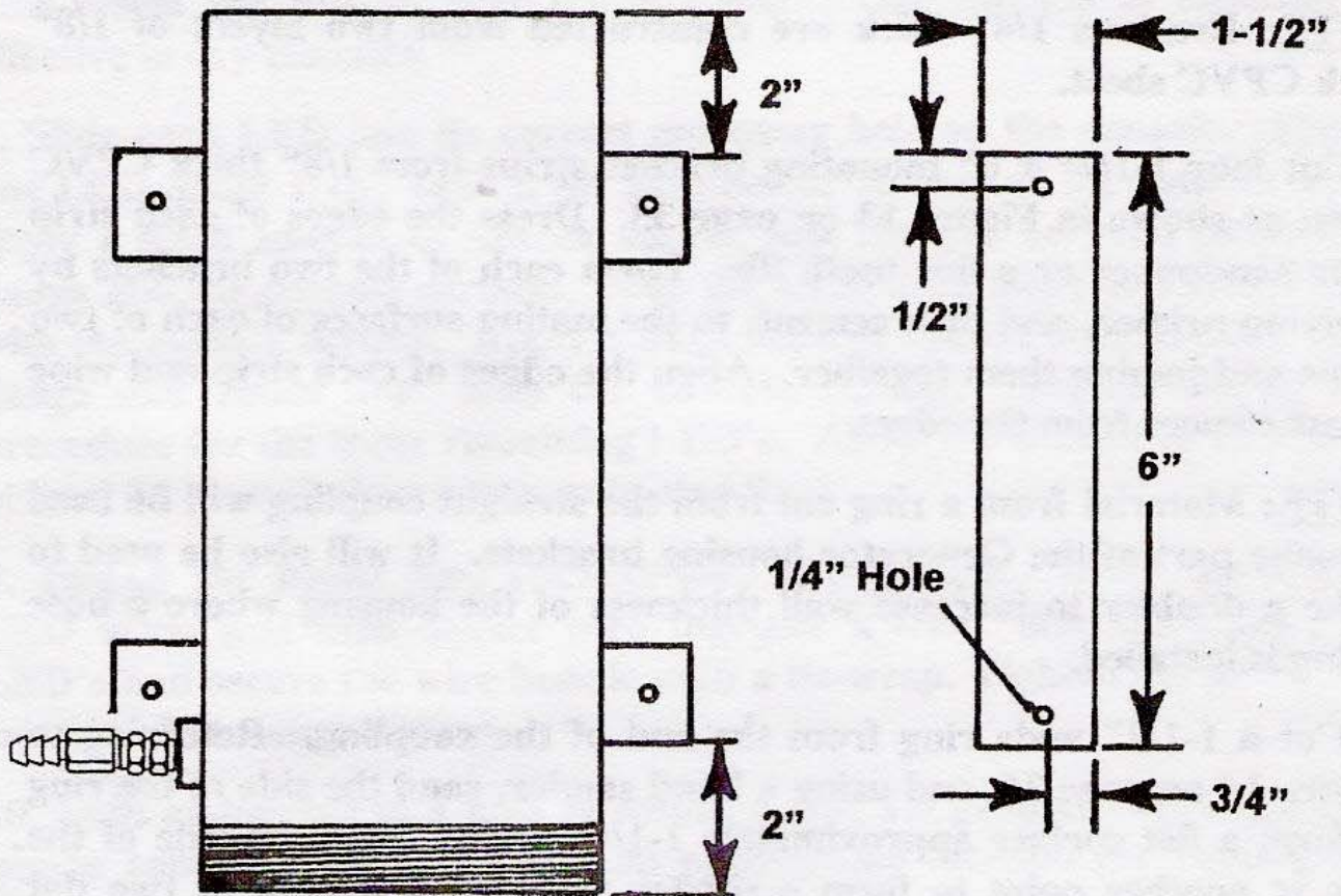
Housing Attachment Details Figure 13
