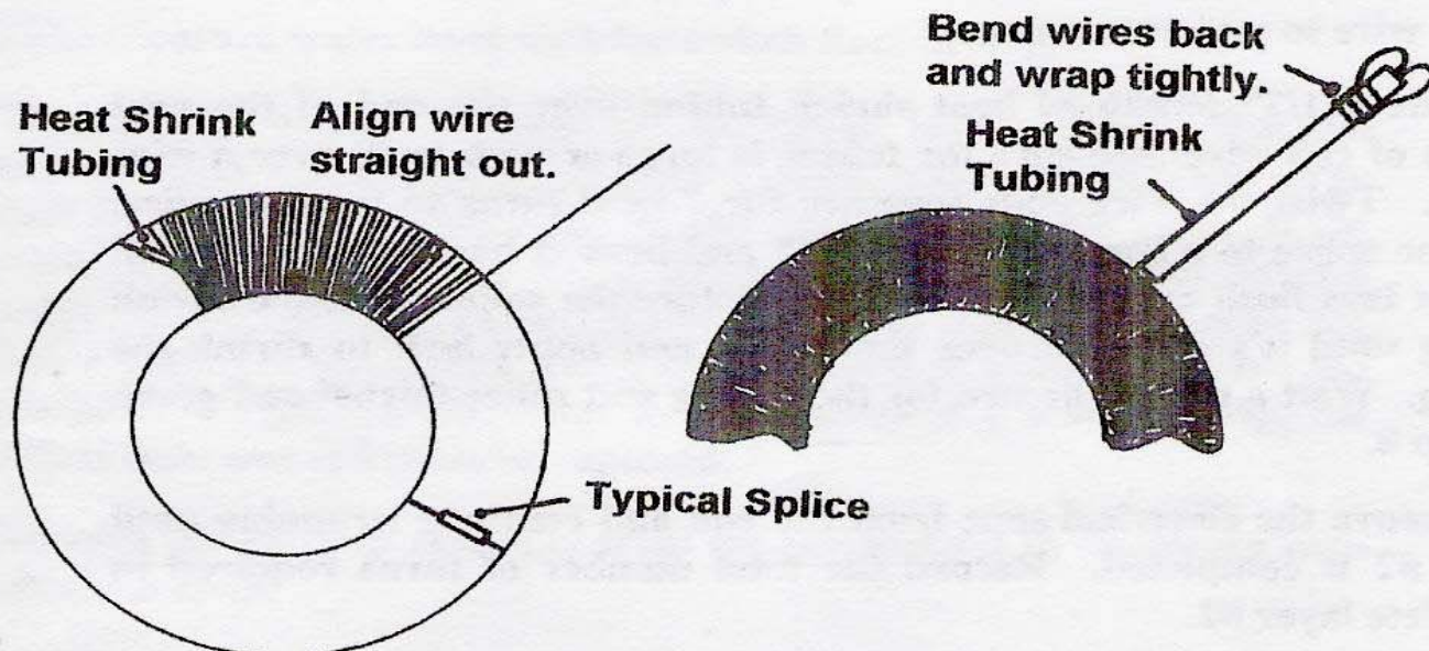
Toroid Coil Details Figure 19
