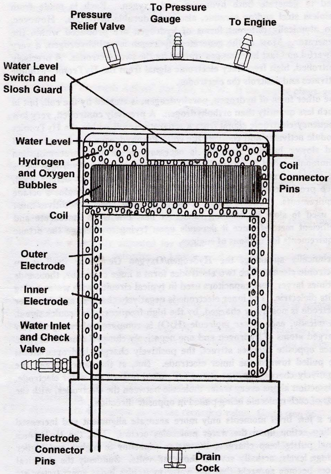
Hydrogen/Oxygen Generator Figure 1
