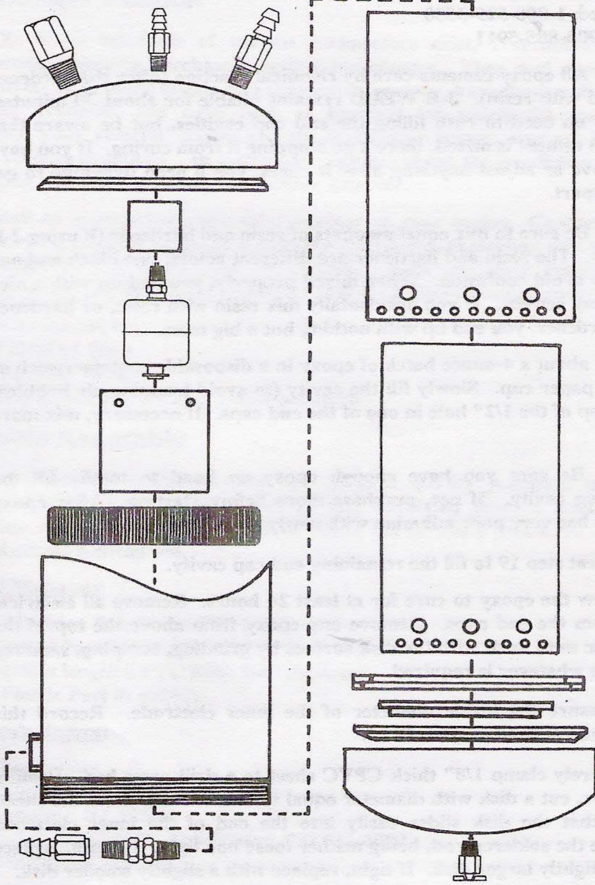
Generator Details Figure 10
