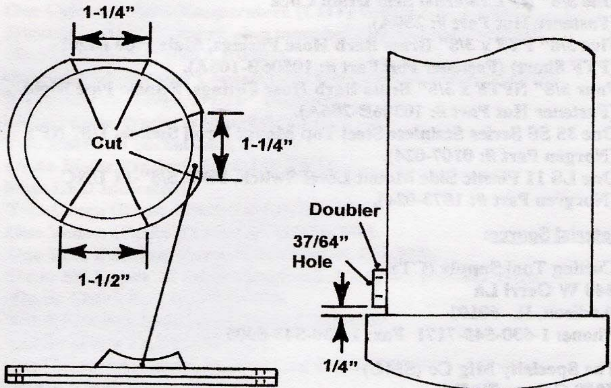
More Housing Attachment Details Figure 14
