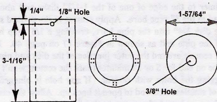
Slosh Shield Details Figure 16
