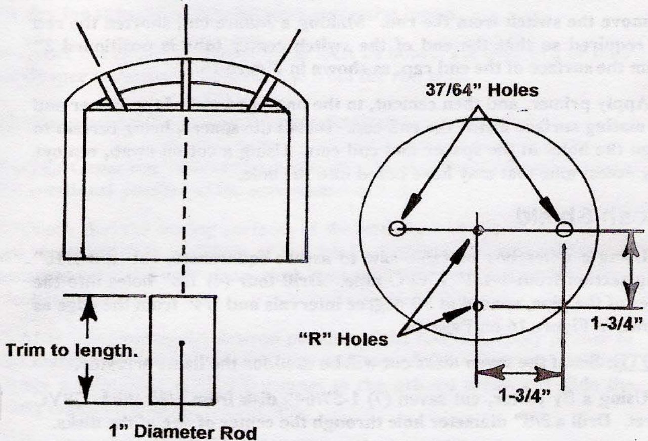
Unthreaded End Cap Details Figure 15
